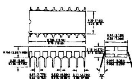
16-PIN Cerdip Package (Suffix Q)
