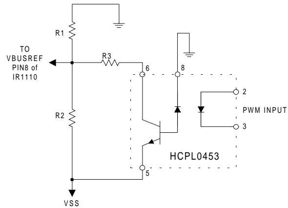
Figure 9 Circuit for PWM Control of DC Bus Voltage
