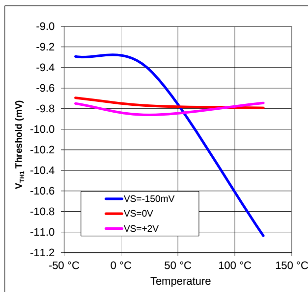
Figure 20: V_{TH1} vs. Temperature and Common Mode (OVT=Floating)
