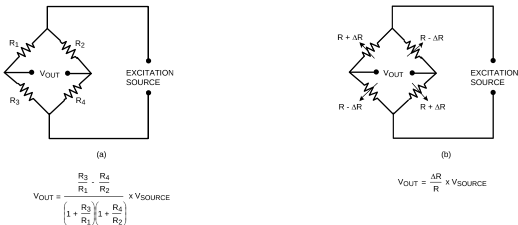
Figure 50. Bridge Sensor
