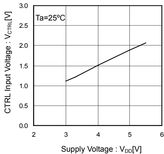
Figure 7. CTRL Input Voltage vs Supply Voltage (BD6516F)
