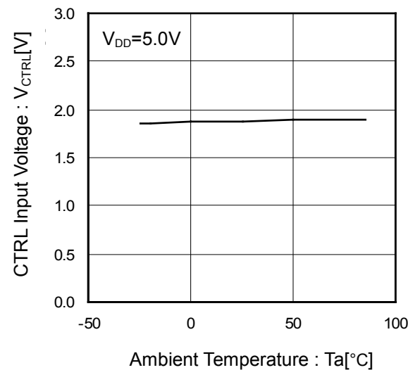
Figure 8. CTRL Input Voltage vs Ambient Temperature (BD6516F)
