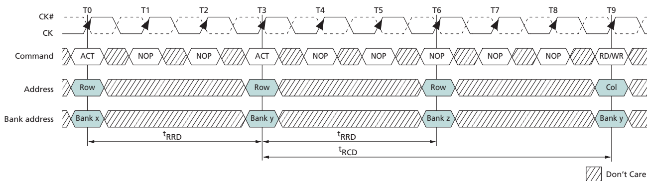
Figure 42: Example: Meeting t_{\text{RRD}} (MIN) and t_{\text{RCD}} (MIN)
