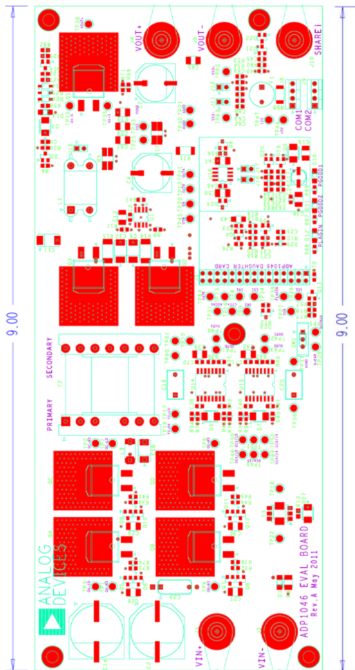
Figure 76 – Layout, Silkscreen layer, dimensions in inches
