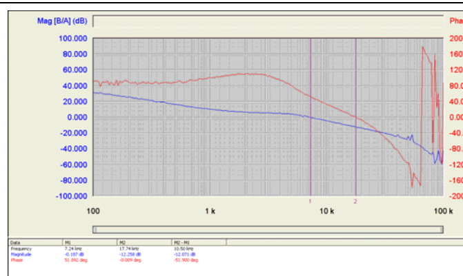
Figure 44 – Digital compensation for CCM. Injected noise of 500mVpp. Crossover frequency at 7.24KHz Phase margin of 51 degrees
