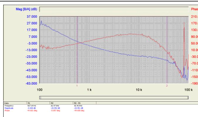
Figure 43 – Loop gain for DCM. Injected noise of 100mVpp. Crossover frequency at 567Hz Phase margin of 50 degrees
