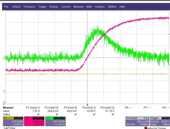
Figure 68 – Feedforward disabled, 8A load Red trace: Input voltage 36-60V Lower trace: AC coupled output voltage
