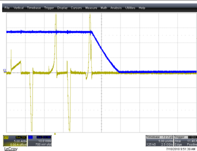
Figure 52 - Synchronous rectifiers shorted, 48VDC, 8A load Upper trace: OrFET gate voltage, 10V/div, 5us/div Lower trace: Primary current, 5A/div, 5us/div
