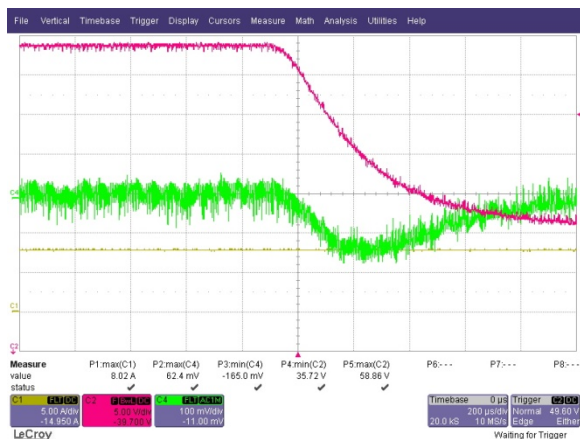
Figure 66 – Feedforward disabled, 8A load Red trace: Input voltage 60-36V Lower trace: AC coupled output voltage
