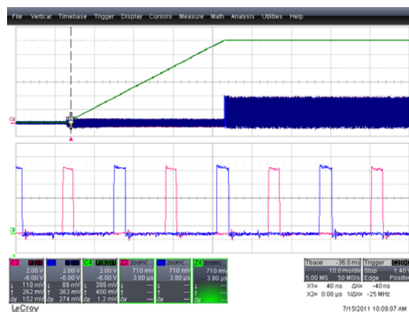
Figure 19 – Progression of SR PWMs during SR softstart Green trace: Output voltage Red trace: SR1 Blue trace: SR2
