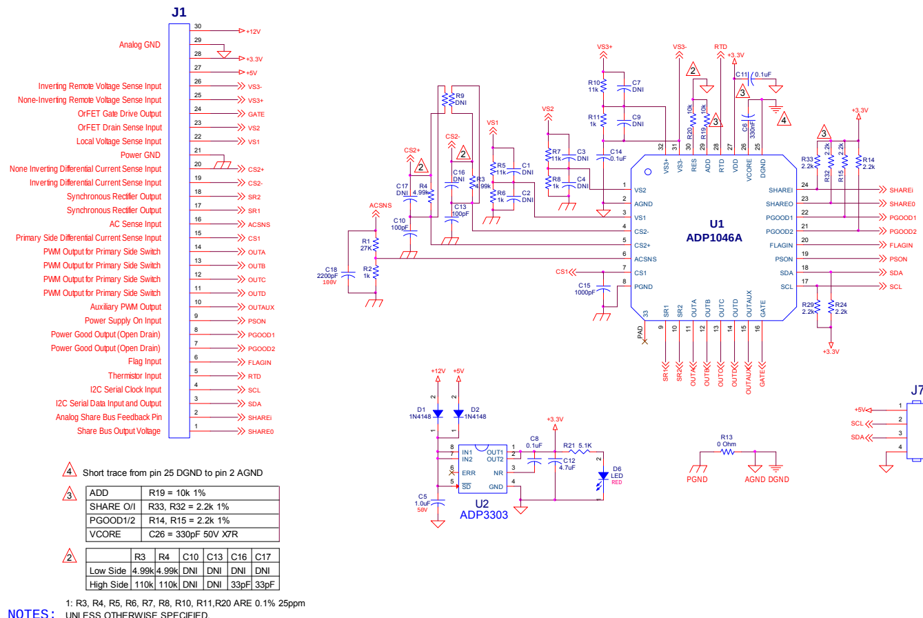
Figure 75 – Daughter card schematic
