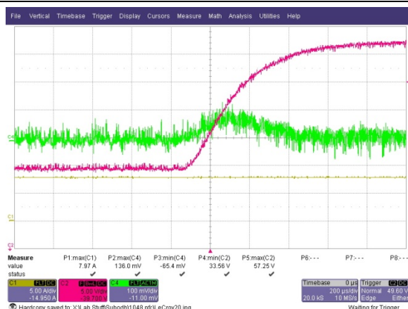
Figure 69 – Feedforward disabled, 8A load Red trace: Input voltage 36-60V Lower trace: AC coupled output voltage
