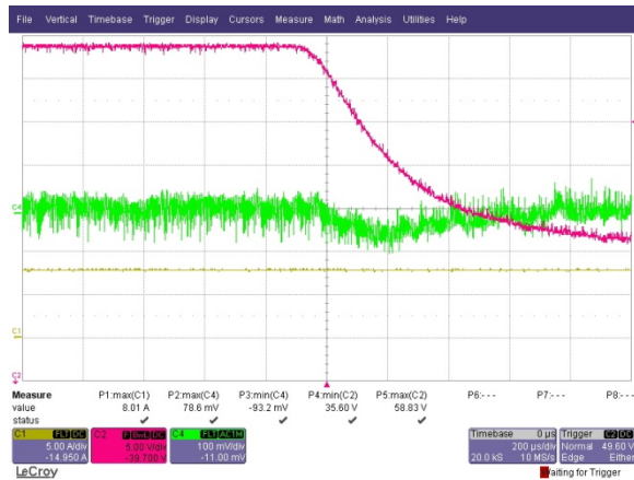
Figure 67 – Feedforward enabled, 8A load Red trace: Input voltage 60-36V Lower trace: AC coupled output voltage
