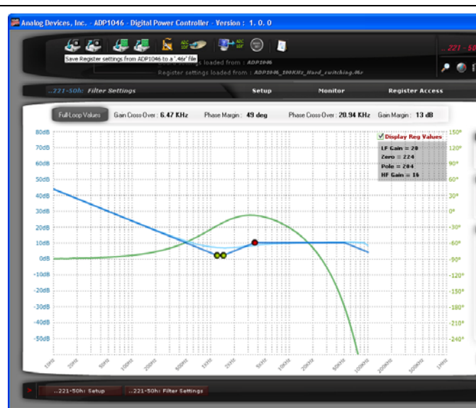
Figure 42 - Digital compensation for normal or heavy load (CCM)
