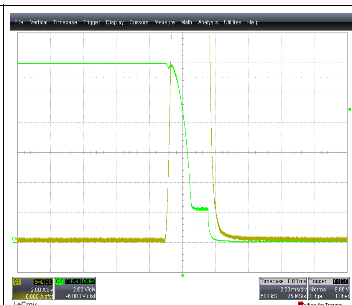
Figure 37 - Under Voltage Protection triggered due to shorted load. Green trace: Output voltage Yellow trace: Load current
