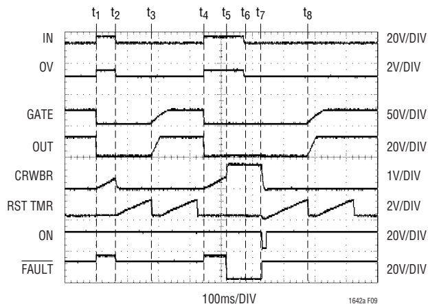
Figure 9. Overvoltage Timing (Input Side)
