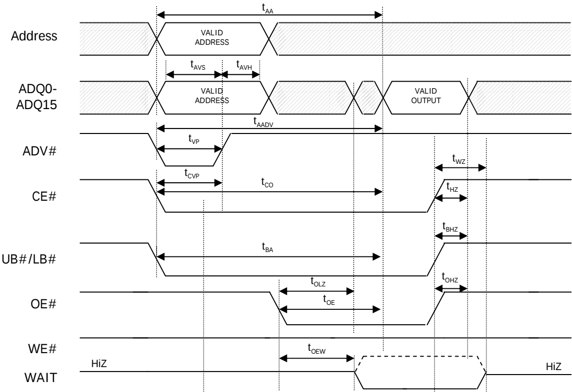
Figure 19: Asynchronous READ
