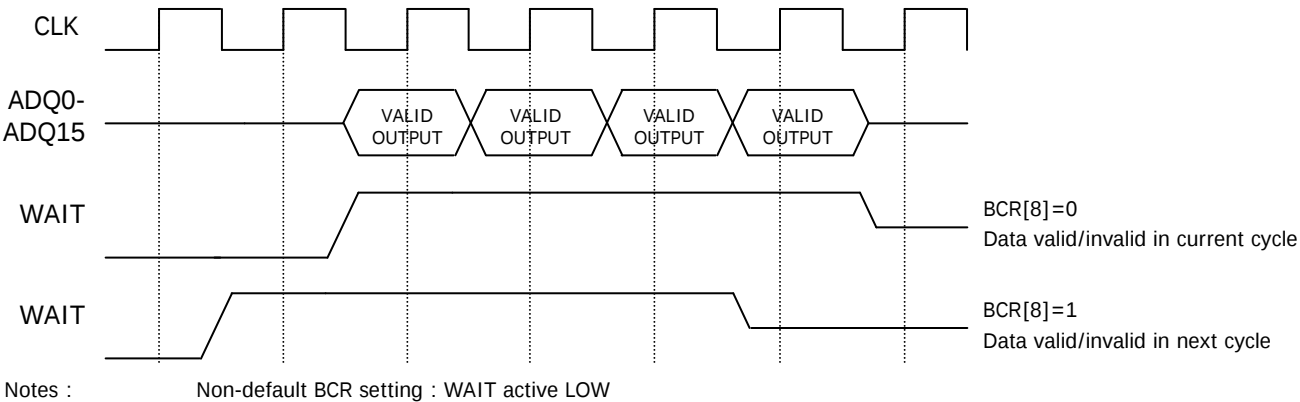
Figure 12. WAIT Configuration During Burst Operation
