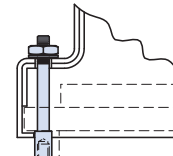
Code FF Fixed Female Jackpost
