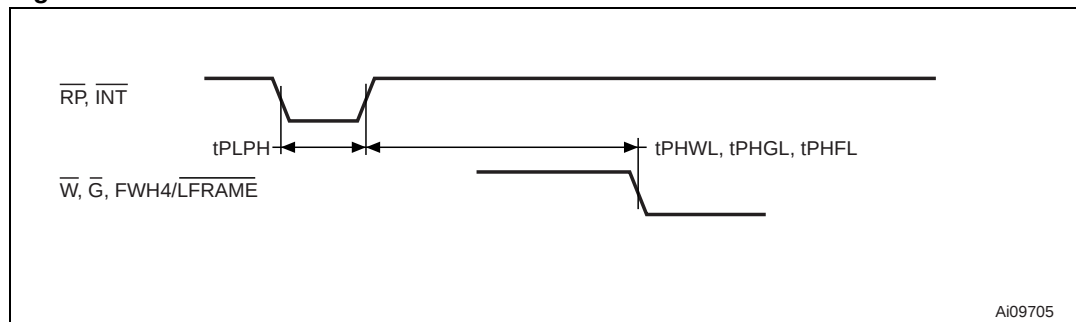
Figure 15. Reset AC waveforms
