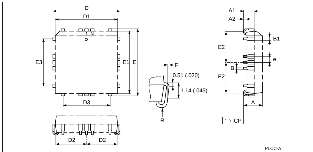
Figure 18. PLCC32 – 32 pin Rectangular Plastic Leaded Chip Carrier, package outline
