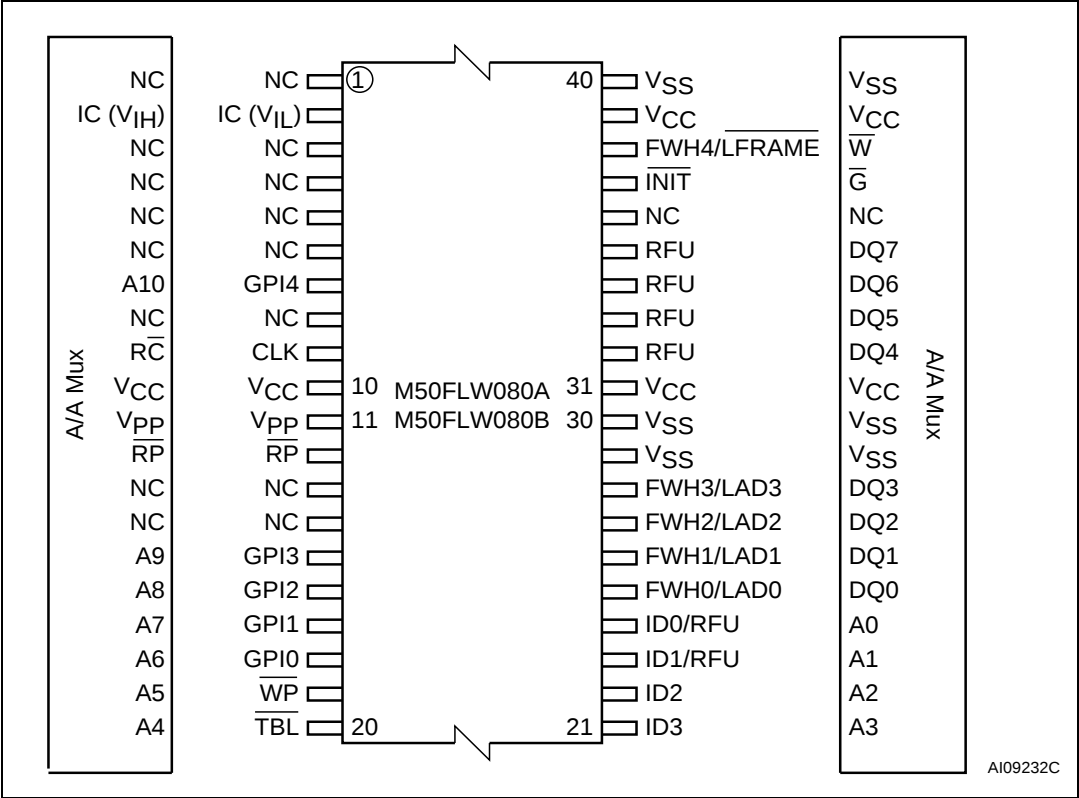
Figure 5. TSOP40 connections
