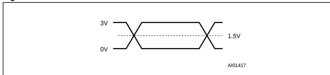
Figure 11. A/A Mux interface AC measurement I/O waveform
