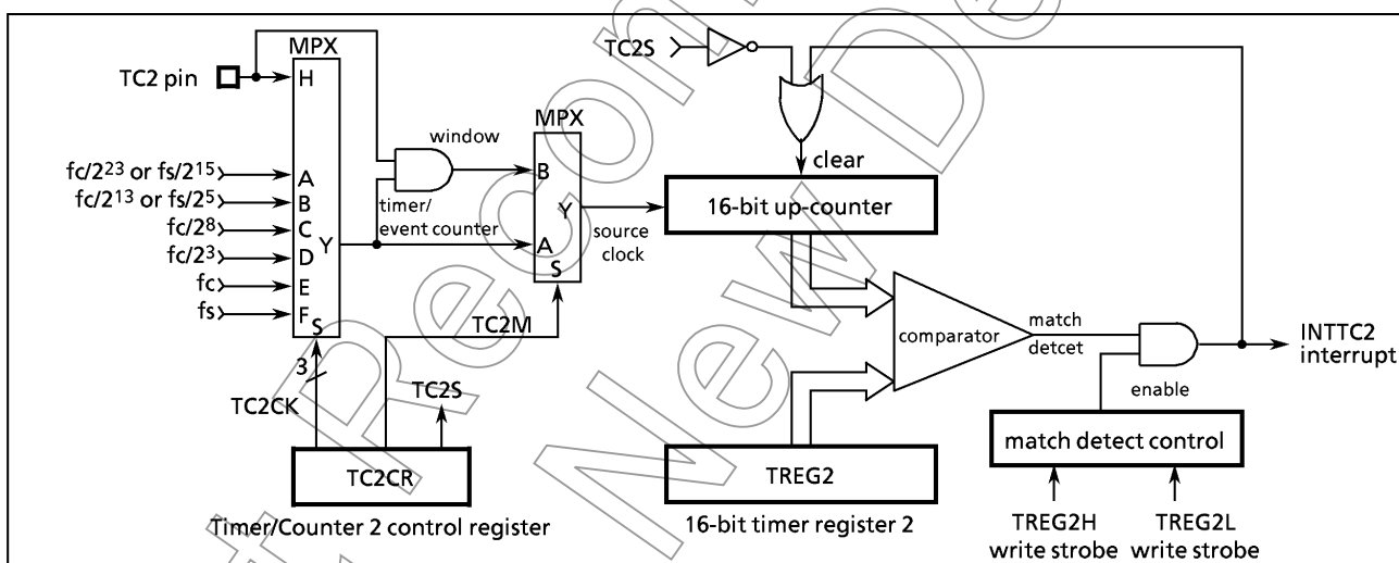
Figure 2-27. Timer/Counter 2 (TC2)
