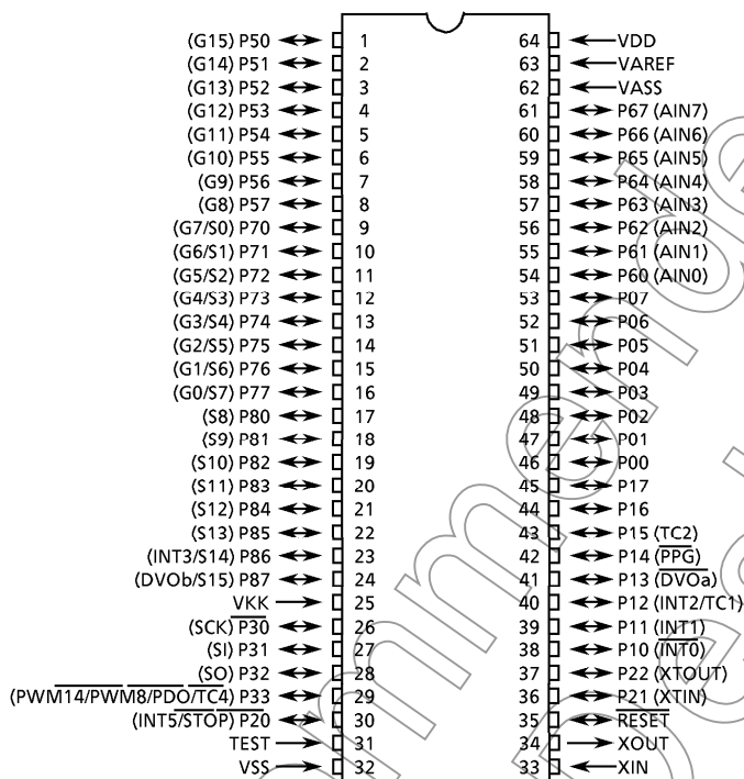
(1) P-SDIP64-750-1.78
