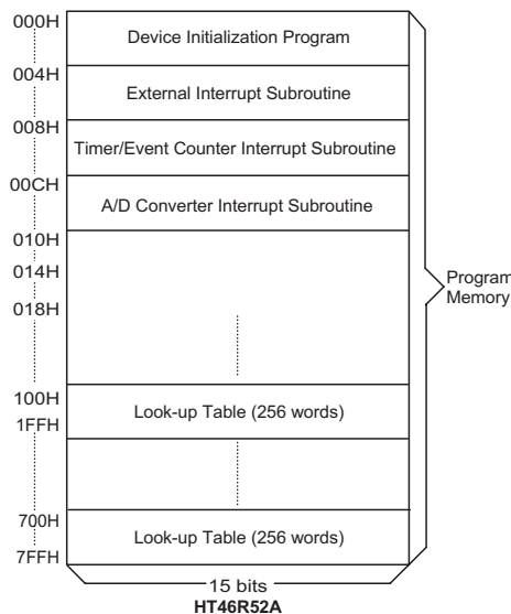
Program Memory
