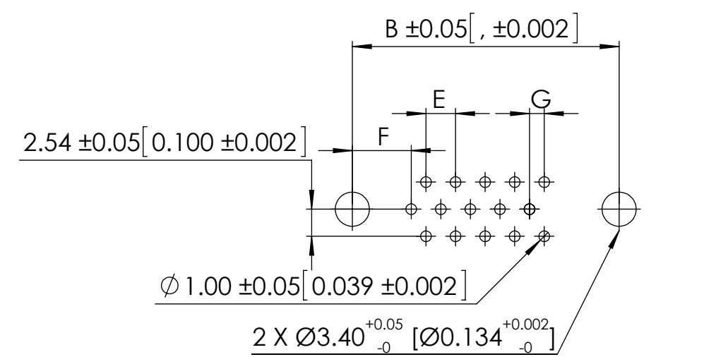
RECOMMENDED PCB LAYOUT 15 POSITIONS MALE
