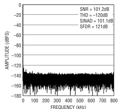
32k Point FFT f_s = 1.6\text{Msps} , f_{\text{IN}} = 2\text{kHz}
