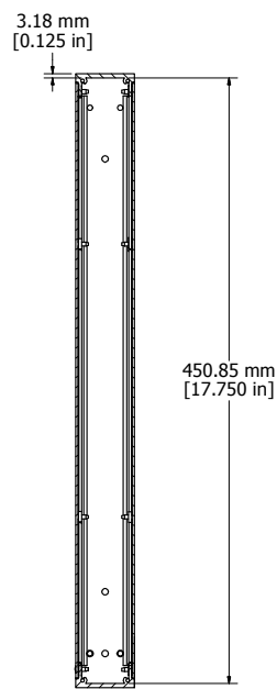
SECTION DD-DD
