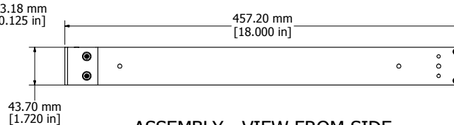
ASSEMBLY - VIEW FROM SIDE
