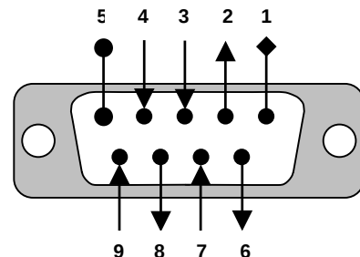
Serial Port Plug connector (female)
