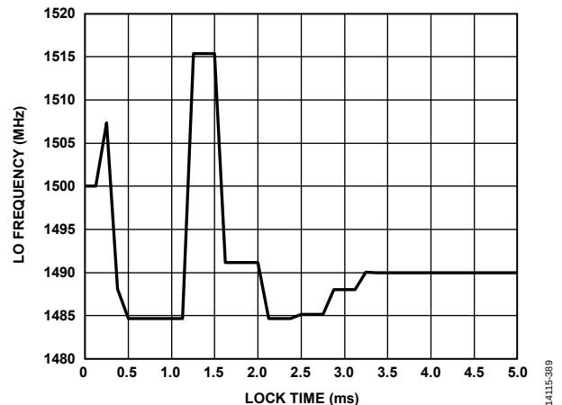
Figure 101. LO Frequency Settling Time, Fractional Loop Filter, Fractional Mode
