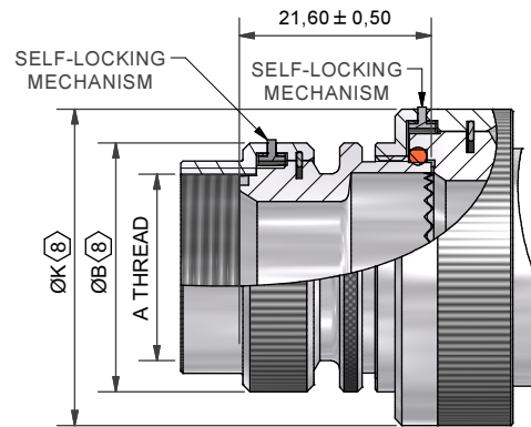
BACKSHELL - TYPE 2
