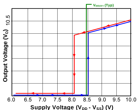
Figure 37. Si823x UVLO Response (8 V)
