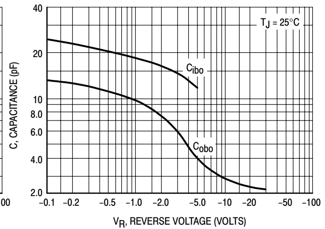
Figure 6. MPS8598/99 Capacitance
