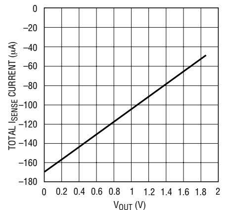
Total I_{SENSE} Current vs V_{OUT}
