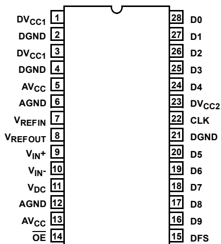
HI5767 (SOIC, SSOP) TOP VIEW
