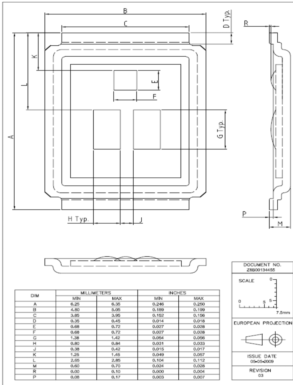
Figure 1 Outlines MG-WDSN-2, dimensions in mm/inches
