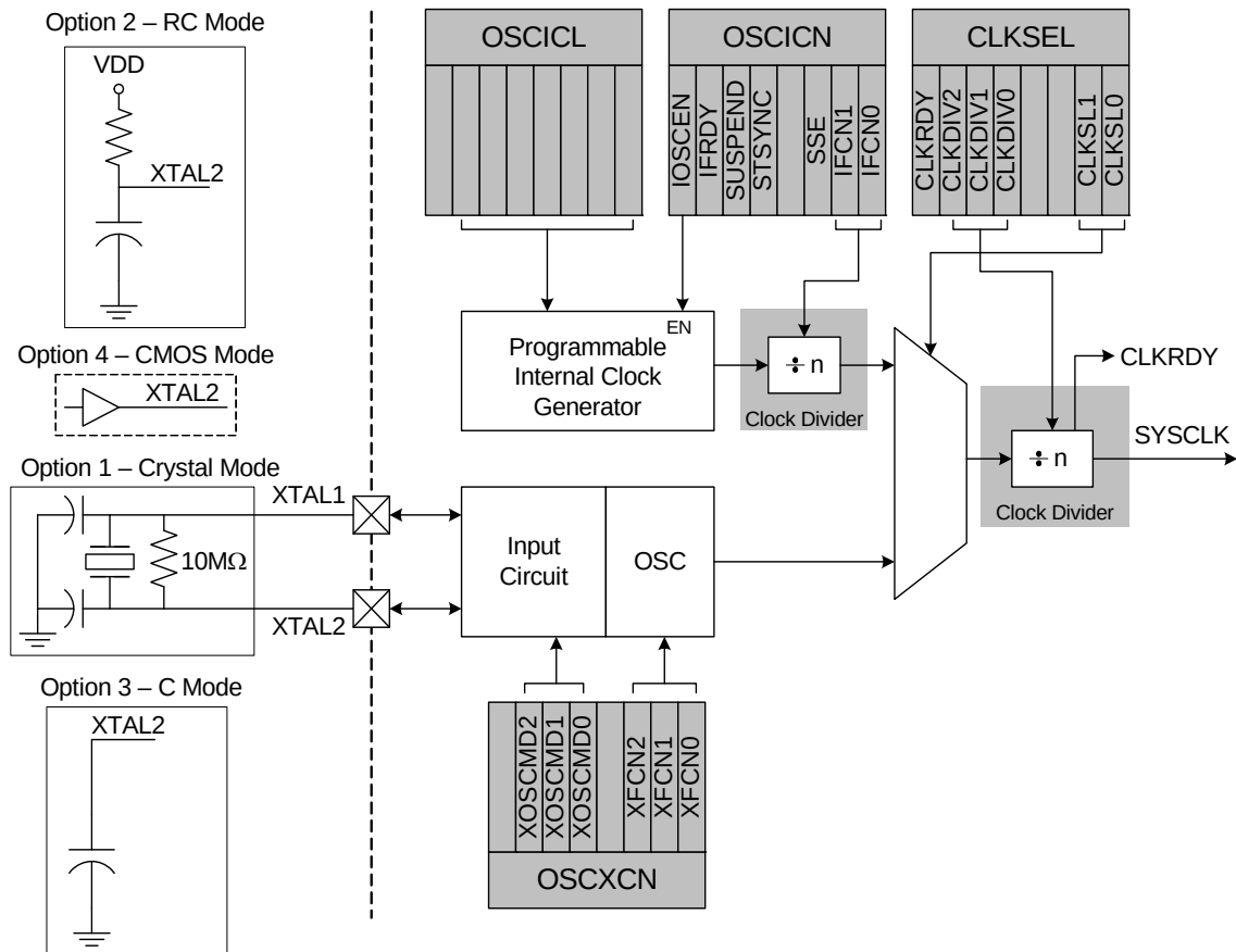
Figure 27.1. Oscillator Options
