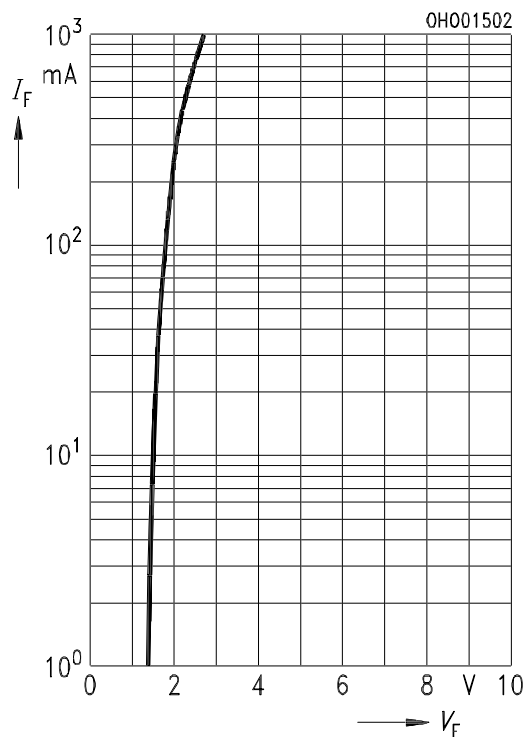
Forward current I_F = f(V_F) , single pulse, duration = 20 \mu\text{s}
