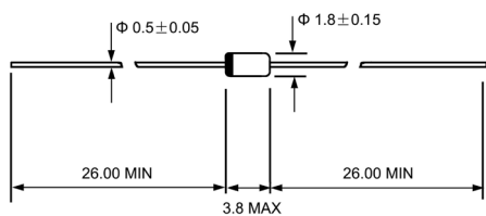
DO-35(GLASS)
