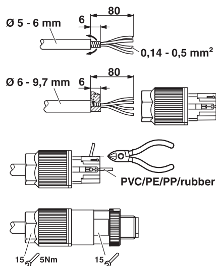
Functional drawing
