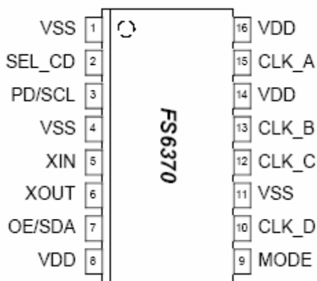
Figure 1: Pin Configuration
