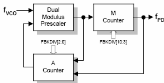
Figure 4: Feedback Divider
