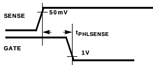
FIGURE 2. SENSE TO GATE TIMING
