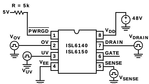
FIGURE 1. TYPICAL TEST CIRCUIT
