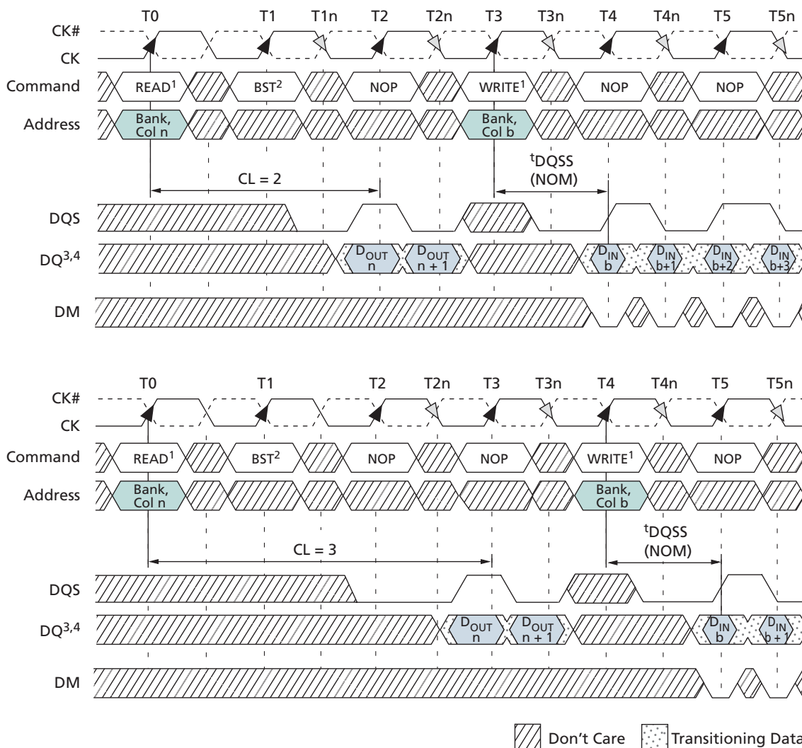
Figure 27: READ-to-WRITE
