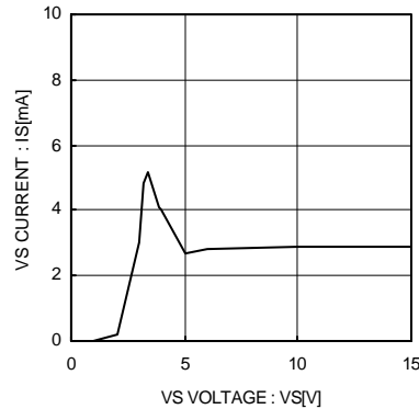
Fig. 17 VS Pin Current
