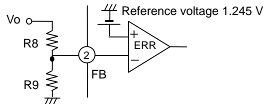
Fig. 31 Feedback Resistance Setting
