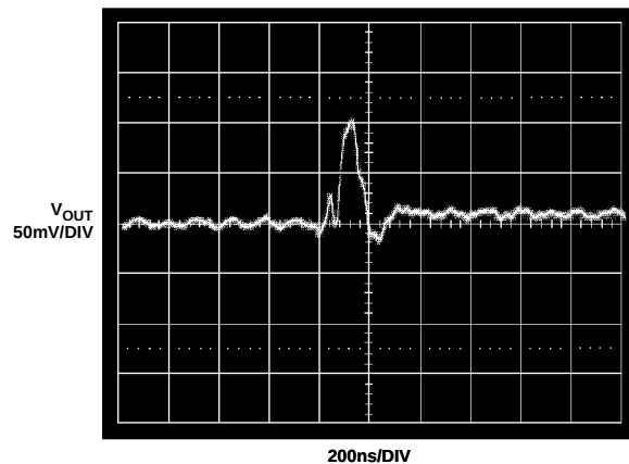
Figure 25. Glitch Impulse
