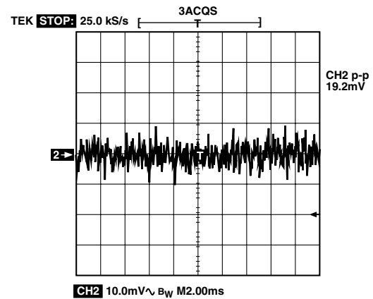
Figure 14a. Peak-to-Peak Full Bandwidth (10 mV/Division)
