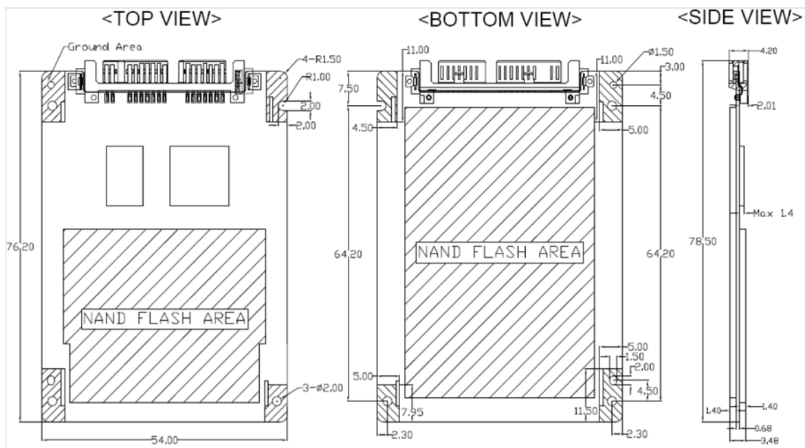
Figure 2-1. Physical dimension
