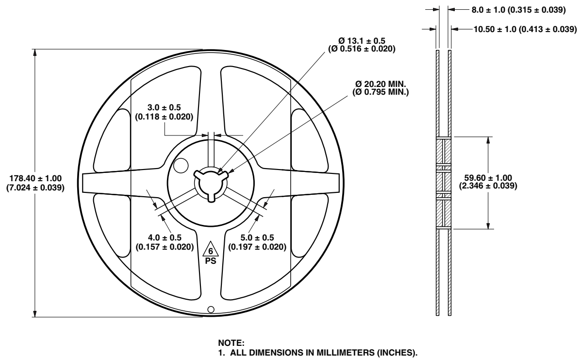
Figure 10. Reel dimensions.
