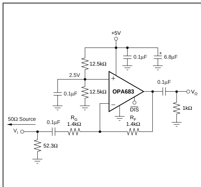
FIGURE 4. AC-Coupled, G = -1V/V , Single-Supply, Specification and Test Circuit.
