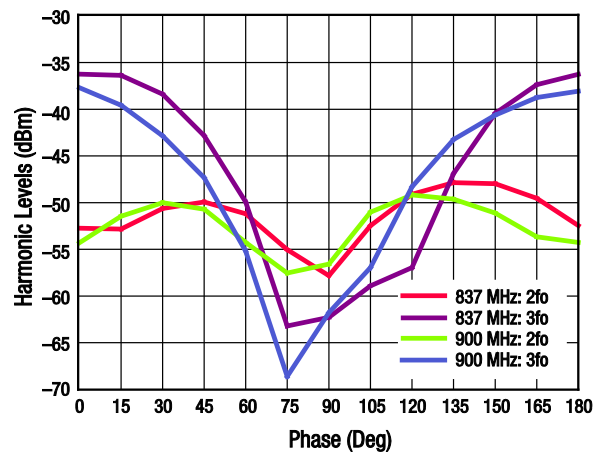
Figure 14. Harmonics vs Phase (ANT to GSM_TX_LB, P_{\text{IN}} = +35 \text{ dBm} , 5:1 VSWR Mismatch)
