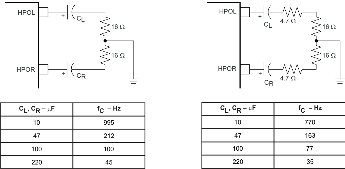
Figure 42. High-Pass Filter for Headphone Output
