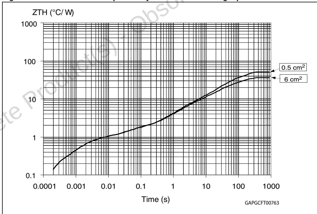
Figure 34. P^2PAK thermal impedance junction ambient single pulse
