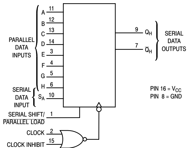
Figure 2. Logic Diagram
