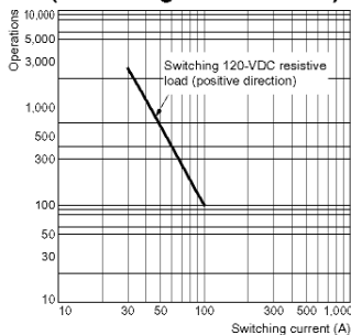
Electrical Endurance (Switching Performance)
