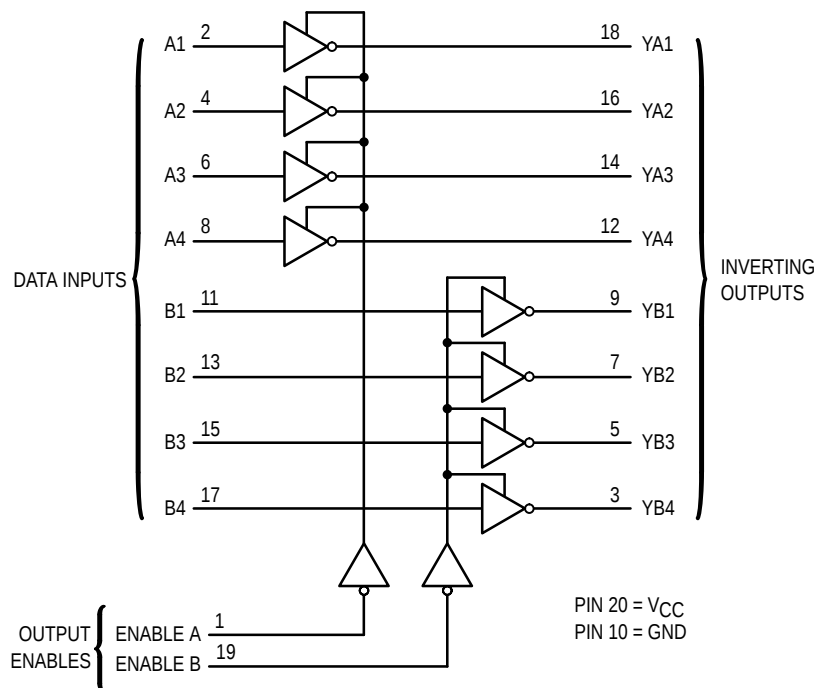
LOGIC DIAGRAM
