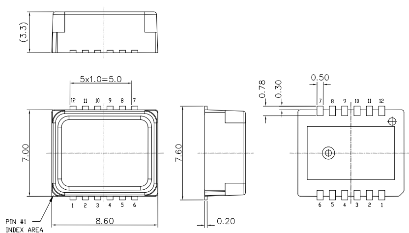
Figure 2. Housing dimensions
