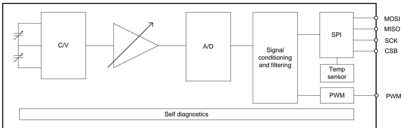
Figure 1. SCA810-D02 Block diagram
