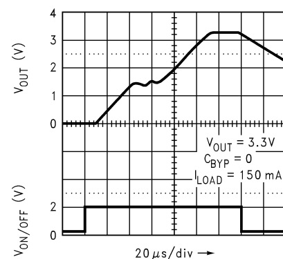
Turn-On Time
