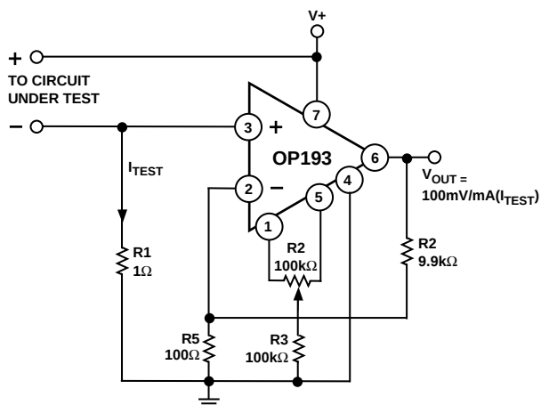
Figure 30. Single-Supply Current Monitor
