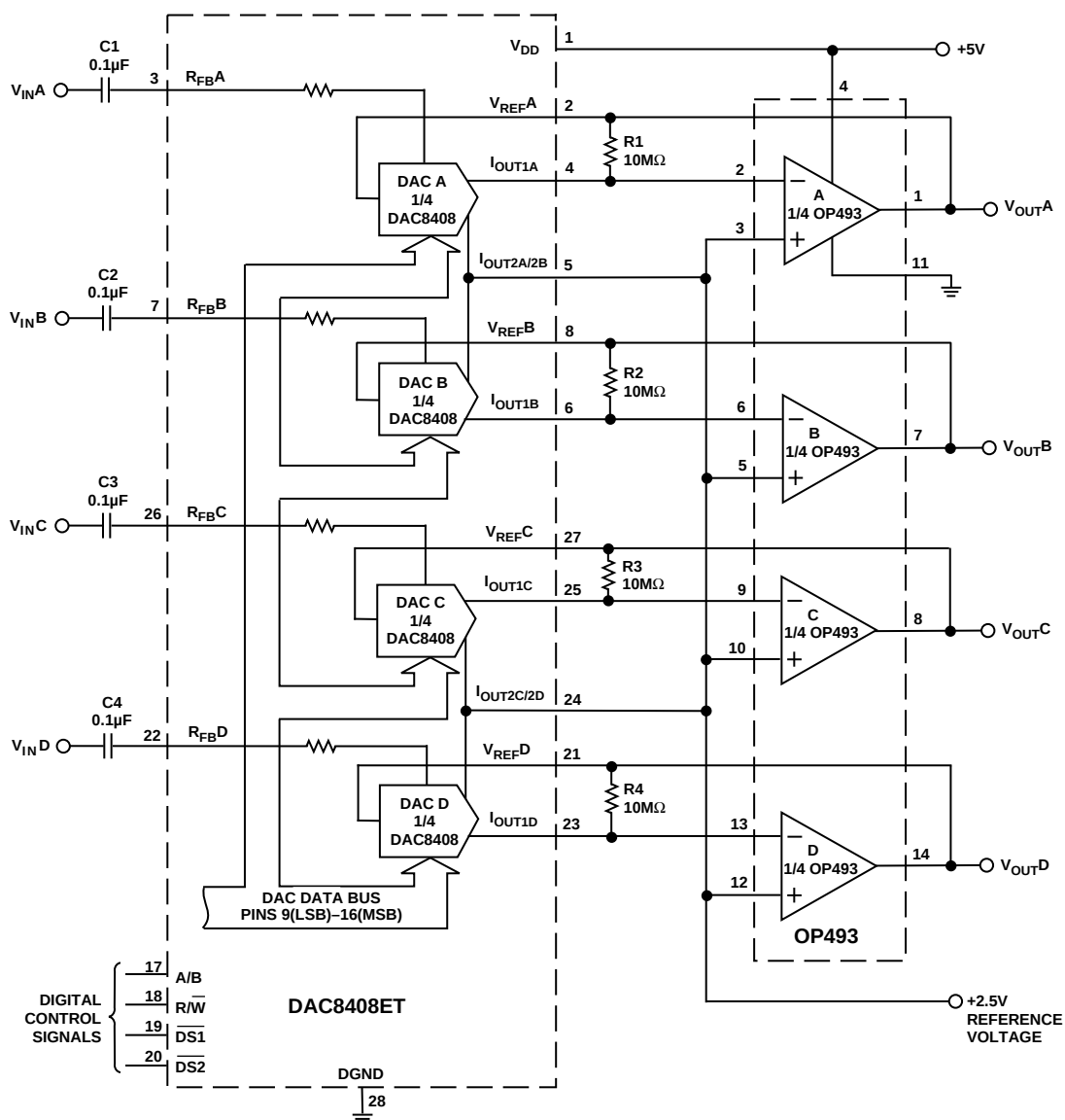
Figure 36. Single-Supply Micropower Quad Programmable-Gain Amplifier
