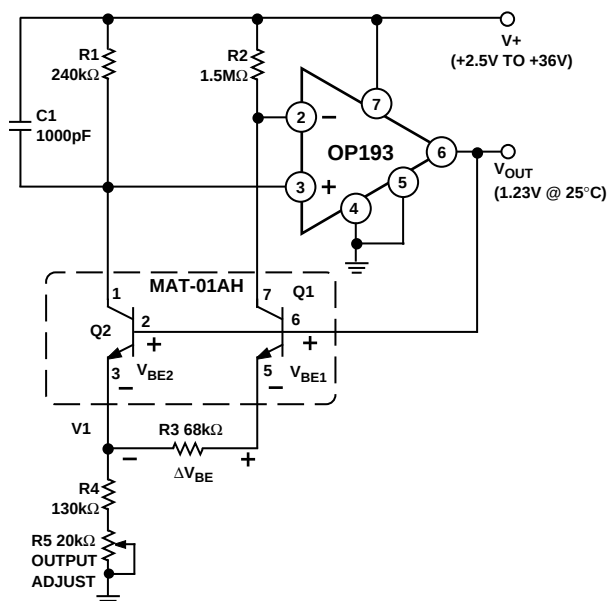
Figure 29. A Battery Powered Voltage Reference
