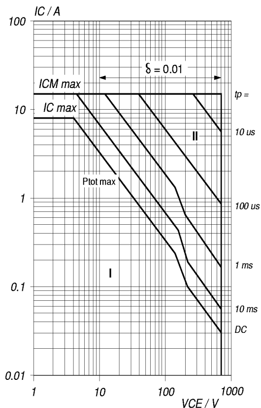
Fig. 13. Forward bias safe operating area. T_{hs} = 25^{\circ}\text{C} I Region of permissible DC operation. II Extension for repetitive pulse operation.
