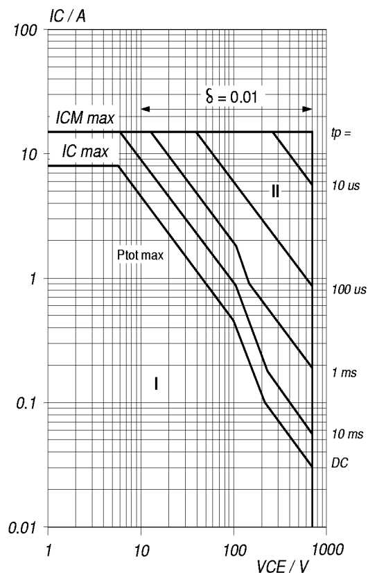
Fig. 12. Forward bias safe operating area. T_{hs} = 25^{\circ}\text{C} I Region of permissible DC operation. II Extension for repetitive pulse operation.
