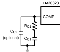
Figure 26. Compensation Network for LM20323
