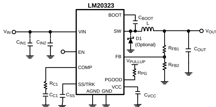
Figure 23. Typical Application Circuit
