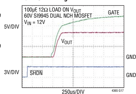
Turn-On Timing
