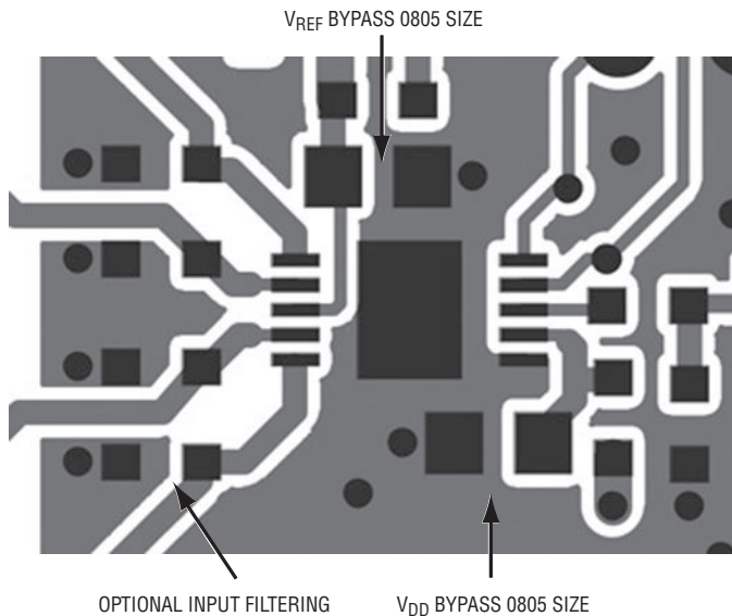
Figure 5. Recommended Layout
