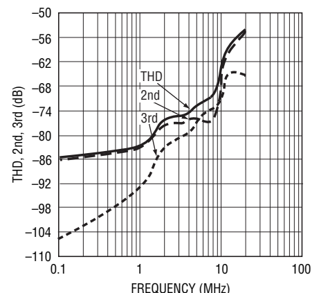
THD, 2nd, 3rd and SFDR vs Input Frequency
